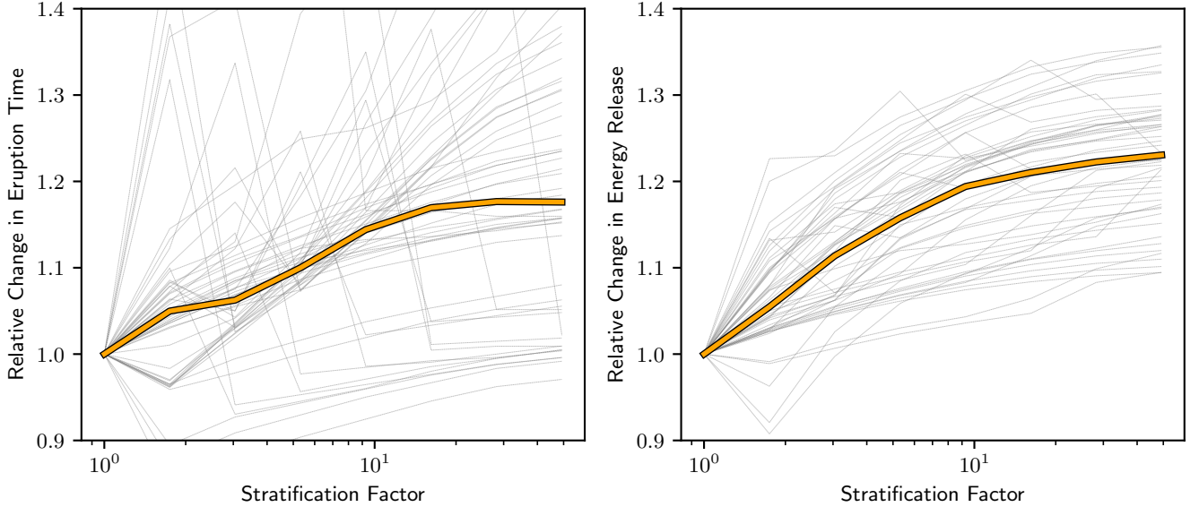
Figure 6. Change in eruption time and energy release with increasing stratification. Each of the thin grey lines represents a sequence of simulations with identical parameters except for the stratification factor. The left pane plots the time taken for an eruption to occur (after the time of the rope’s formation) and the right pane plots the magnetic energy released in the eruption. The grey lines are then normalised by the time/energy of the respective unstratified case. The median values are plotted as the thick orange lines.
