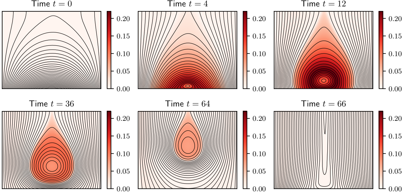
Figure 3. Sequence of snapshots showing a flux rope forming and erupting. The heatmap represents the strength of the out-of-plane magnetic field, and the black lines are the projection of the the magnetic field lines into the plane. The flux rope has already formed by the time of the second snapshot, and erupts shortly after the fifth snapshot at around time t = 65 . In this simulation the stratification factor is S = 150 and the other variable parameters are \eta_0 = 2.36 \times 10^{-3} , \epsilon_0 = 2 .
