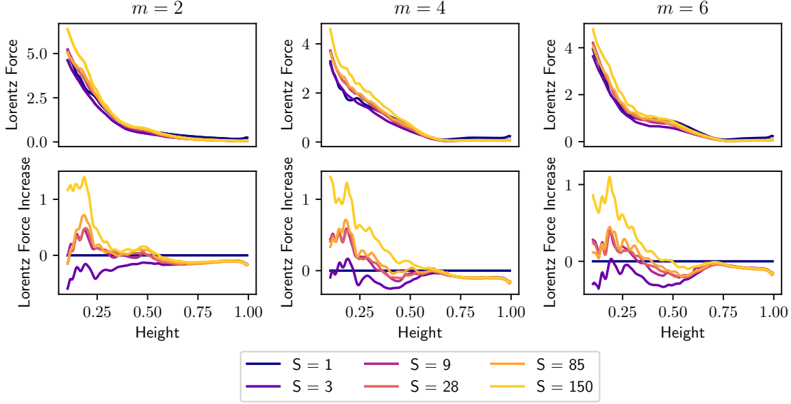
Figure 7. 1D Fourier transforms of the absolute Lorentz Force, at a given height y . The upper pane shows the absolute values of the quantity L_m(y) , for each of the stratification factors averaged over all simulation runs. The lower pane plots these quantities relative to the unstratified case with S = 1 .
