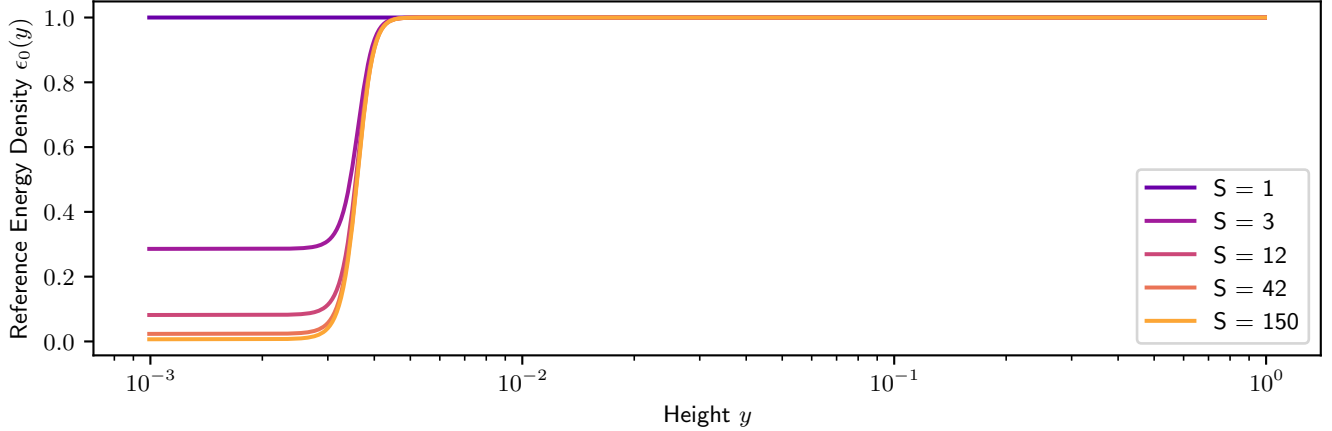
Figure 1. Reference energy density functions \epsilon_0(y) , for varying stratification factors S = 1/T_b . Note the logarithmic scale on the x axis – the function is constant throughout almost the entire domain.
