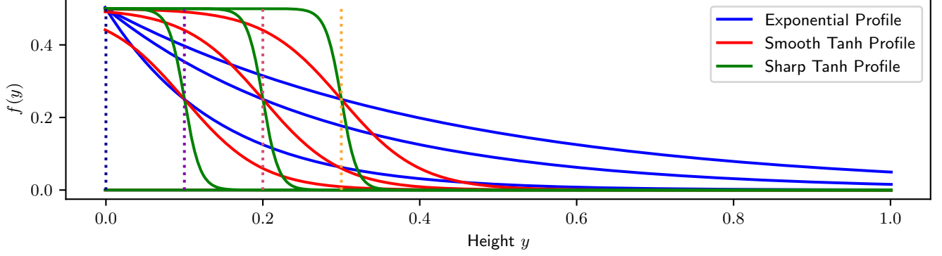
Figure 8. Plot of the three forms of the pressure functions we consider, with f_{\text{exp}}(y) in blue, f_{\text{smooth}}(y) in red and f_{\text{sharp}}(y) in green. The three nonzero profiles of each form correspond to the cutoff height y_0 at which the pressure function decays to half of its value at the base of the domain.
