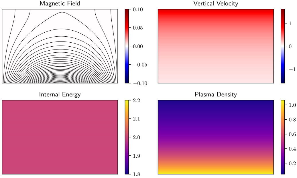
Figure 2. Initial conditions for the MHD simulations. The magnetic field is 2 dimensional, with the lines representing the magnetic field lines in the plane. The initial internal energy is a constant.
