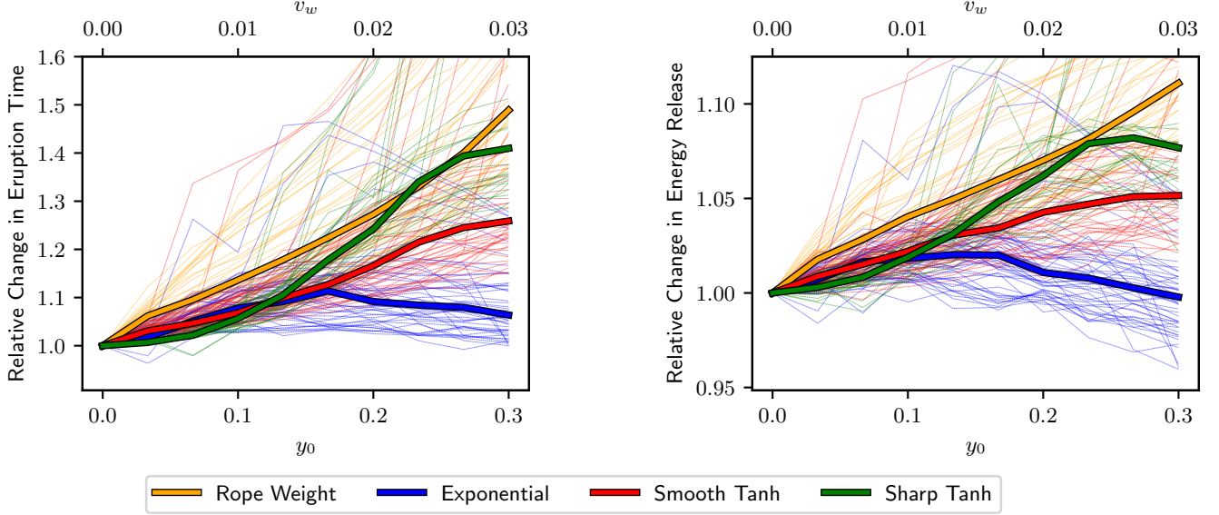
Figure 11. Plots of the delays in the time of flux rope eruptions and the respective releases in magnetic energy, as in Figure 6. All three modifications to the MF model are plotted, and are coloured respectively. All individual simulation sets are plotted as the thin lines, with the median values plotted as the thick outlined lines.
