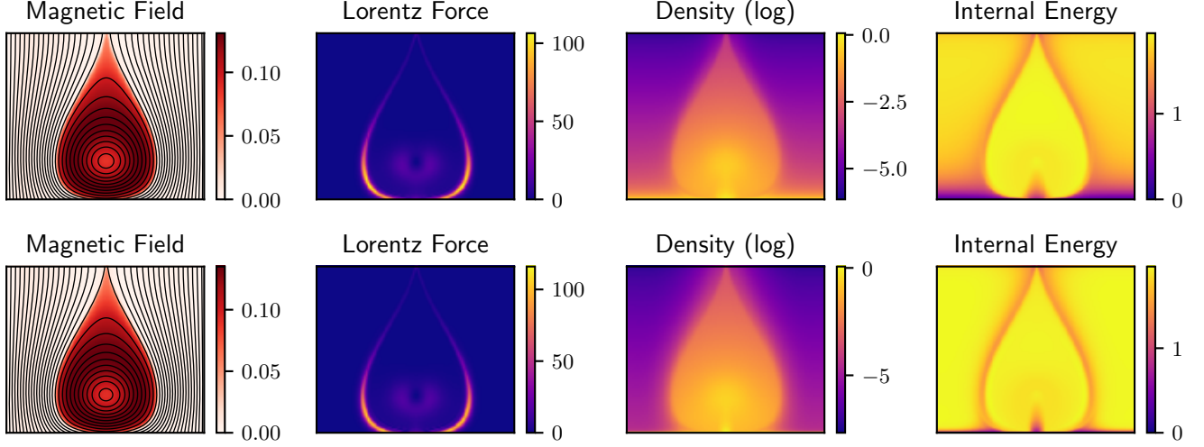
Figure 4. Comparison of an unstratified (top) and stratified (bottom) simulations at the same time during flux rope formation, with all other parameters identical. This is a snapshot at time t = 16 . The lower pane is the same simulation as shown in Figure 3, and the upper is the unstratified equivalent with S = 1 . The magnetic field is represented as in Figure 3, and the fluid density is plotted on a logarithmic scale as it varies over several orders of magnitude.
