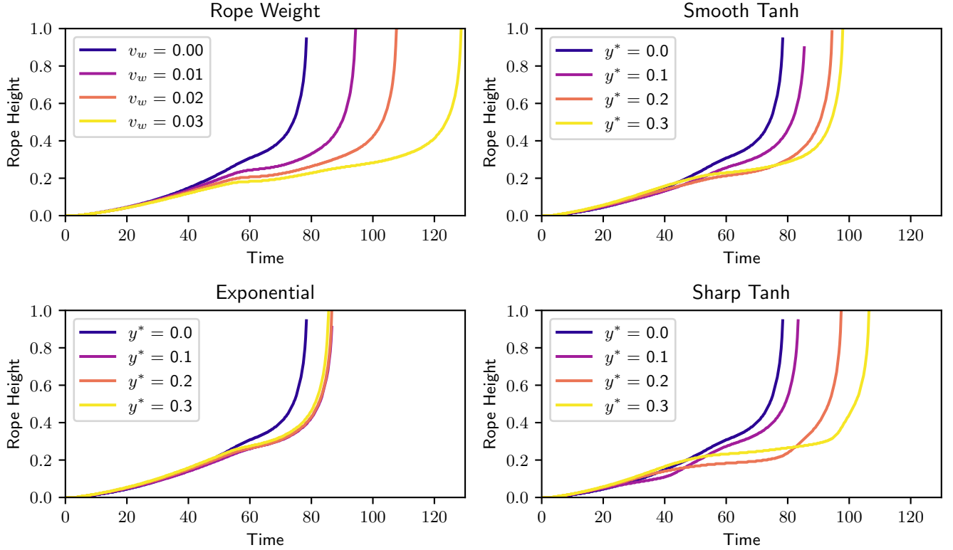
Figure 9. Plots of the height of the centre of the flux rope from the simulations with \eta_0 = 0.001, \nu_0 = 0.06 , showing the delay in eruption due to the effect of the three modifications to magnetofriction that we test. The runs are colour coded based on the modification parameters used in each case.
